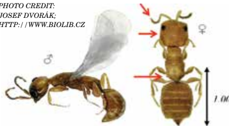
Cephalonomia gallicola : a Bethylid wasp called 'Flat Wasps' in Germany and 'Ant Bees' in Japan.
